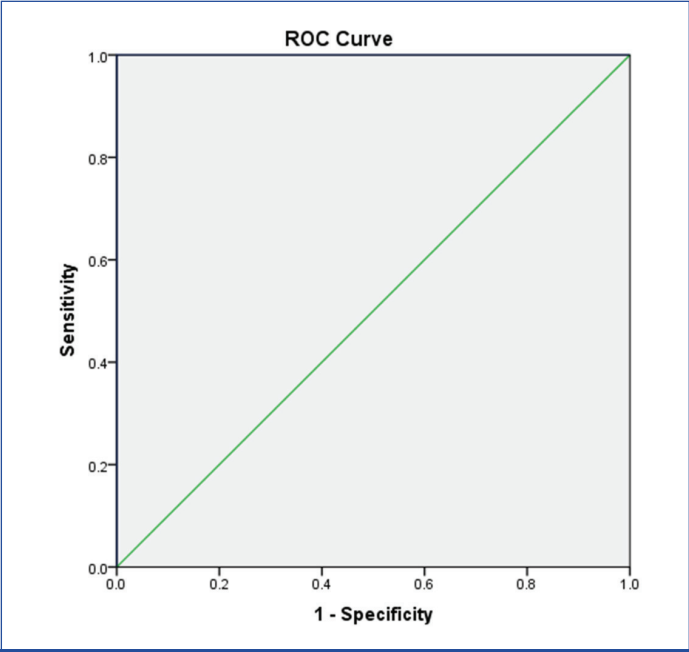
[Table/Fig-1]: ROC analysis showing the cut-off for SII as 581 for 98% sensitivity and 100% specificity (CI=95%, AUC=1).
