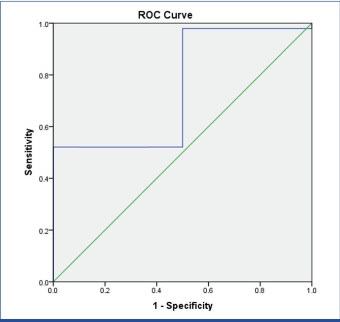
[Table/Fig-2]: ROC analysis showing cut off of SIRI, 0.910 for 96% sensitivity and 50% specificity (CI=95%, AUC=0.750).
